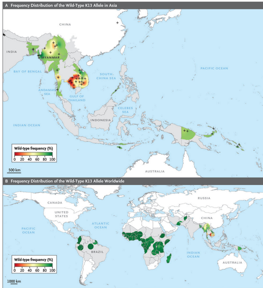
Figure 2. Frequency Distribution of the Wild-Type K13 Allele Shown are the distributions of the wild-type K13 allele in Asia (Panel A) and around the world (Panel B). Areas in which malaria is endemic are shaded in gray, and areas that are considered to be malaria-free are shown in white. The mean frequency of the wild-type allele is indicated by the color code. In Panel A, the individual sites of sample collection are indicated with a cross. In Panel B, a 100-km radius was used for the area centered on each sampling site or on the capital city of the country if no specific site was used for sampling. Data regarding sampling methods and K13 diversity according to country are provided in Tables S4, S5, and S7 and Fig. S3 in the Supplementary Appendix.
