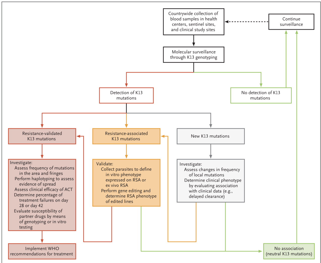
Figure 4. Algorithm for Surveillance of Artemisinin Resistance on the Basis of K13 Mutations Shown is a step-by-step procedure for acquiring information to help develop policies regarding the use of artemisinin-based combination therapy (ACT) and strategies to eliminate malaria. K13 genotyping is integrated into surveillance activities by combining clinical efficacy studies with in vitro susceptibility testing and is supported by gene-editing studies. The validated or confirmed K13 mutations that are associated with resistance to artemisinins are Y493H, R539T, I543T, and C580Y, and the associated K13 mutations are P441L, F446I, G449A, N458Y, P553L, R561H, V568G, P574L, and A675V. 3 The validation of a K13 mutation as a resistance marker (i.e., confirmed K13 mutation) is based on the following criteria: a significant association with delayed clearance of Plasmodium falciparum and a reduced drug sensitivity (survival rate, >1%) on ex vivo ring-stage survival assay (RSA) or in vitro RSA performed on field isolates, culture-adapted parasites, or gene-edited parasite lines, as compared with the K13 wild-type parent control. A K13 mutation is deemed to be associated with artemisinin resistance if it has a significant association with delayed clearance. A K13 mutation is said to be neutral if it has no significant association with delayed clearance or reduced drug sensitivity. A new K13 mutation is one that has been
