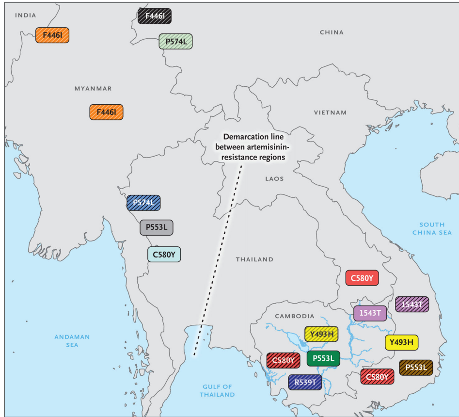
Figure 3. Overview of the Distribution of the Flanking Haplotypes of the C580Y, Y493H, R539T, I543T, P553L, P574L, and F446I Nonsynonymous Mutations in K13 in Two Regions in Asia Shown are two areas in Asia in which individual K13 nonsynonymous mutations (which are labeled in the colored boxes) were frequently identified: one area that includes Cambodia, Vietnam, and Laos and a second area that includes western Thailand, Myanmar, and China. The haplotype groups of C580Y, F446I, P574L, and P553L are shown in distinct colors. Similarly colored boxes indicate shared haplotypes, and hatched boxes indicate the presence of additional countryspecific haplotypes. For example, C580Y haplotypes that are shared between Cambodia, Vietnam, and Laos (H29, H33, or H43) are shown in red, whereas the C580Y haplotype found in Thailand (H42) is shown in light blue. Full details about the distribution of haplotypes are provided in Table S9 and Fig. S9 in the Supplementary Appendix.
