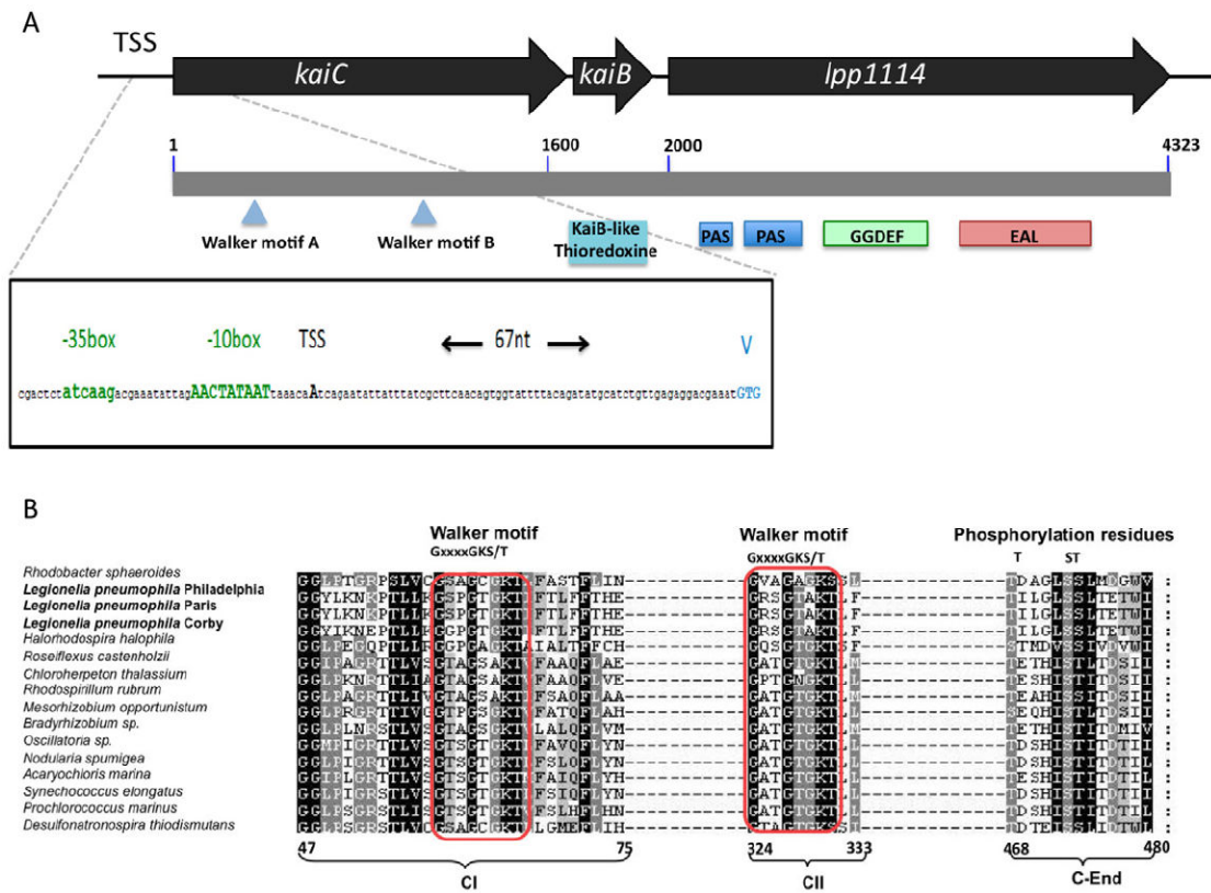
Fig. 1. Schematic representation of the kai operon in Legionella pneumophila .
