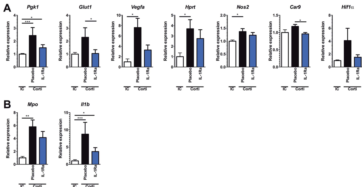
Figure 4. IL-1Ra (Anakinra) treatment reduces expression of hypoxia inducible transcripts. (A–C) mRNA expression in lung homogenates at day 3 p.i. of Aspergillus -infected immunocompetent (IC) and corticosteroid immune suppressed mice (Corti) mice, that were either placebo treated or treated with IL-1Ra (Anakinra). mRNA expression of (A) the hypoxia inducible genes Pgk1 , Glut1 , Vegfa , Hprt , Nos2 , Car9 (B) their transcription factor Hif1α and (C) inflammatory genes Mpo and Il1b was assessed and normalized against housekeeping gene Gapdh . The expression is relative to the expression in the immunocompetent group which was set at 1 \pm \text{SEM} . Data is represented as mean \pm SEM and were compared for significance using the Mann-Whitney U test. *p < 0.05; **p < 0.005; ***p < 0.001.
