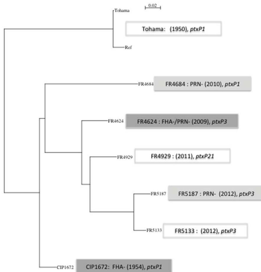
Figure 1. Phylogenetic tree based on 337 SNP. 337 SNP (comprising all SNPs found in all tested isolates) were concatenated using SynTview ( http://genopole.pasteur.fr/SynTVView/ ). Alignment was done using multalin ( http://multalin.toulouse.inra.fr/multalin/ ) and the phylogenetic tree was done using Quicktree ( http://mobyle.pasteur.fr/cgi-bin/portal.py?forms::quicktree ).
