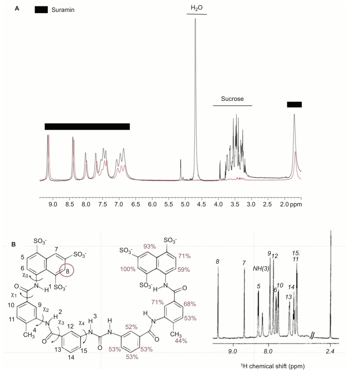
Figure 4 STD NMR assay of suramin-EV71 particle binding. (A) STD NMR of suramin with the EV71 particle. ^1\text{H} (proton) NMR spectrum of suramin, shown in black, and STD NMR spectrum of suramin in complex with EV71 particles, shown in red. (B) Left: structure of suramin, labeled with proton positions and relative intensity percentages. Right: ^1\text{H} NMR spectrum of suramin, with proton numbers shown.
