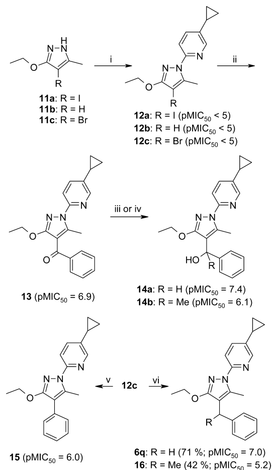
Scheme 1 a
