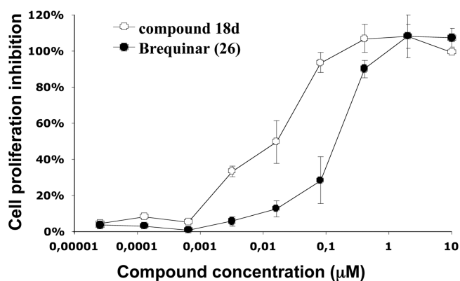
Figure 6. Inhibition (%) of Jurkat cells proliferation by compound 18d and brequinar ( 26 ). Jurkat cells were incubated with increasing doses of 18d or brequinar. As a control, cells were treated with DMSO alone. At t = 0 and after 72 h of culture, the number of living cells was determined using the CellTiter-Glo reagent. The inhibition of cellular proliferation is expressed as a percentage relative to DMSO-treated control wells. The results presented correspond to the mean \pm SD of two independent experiments.
