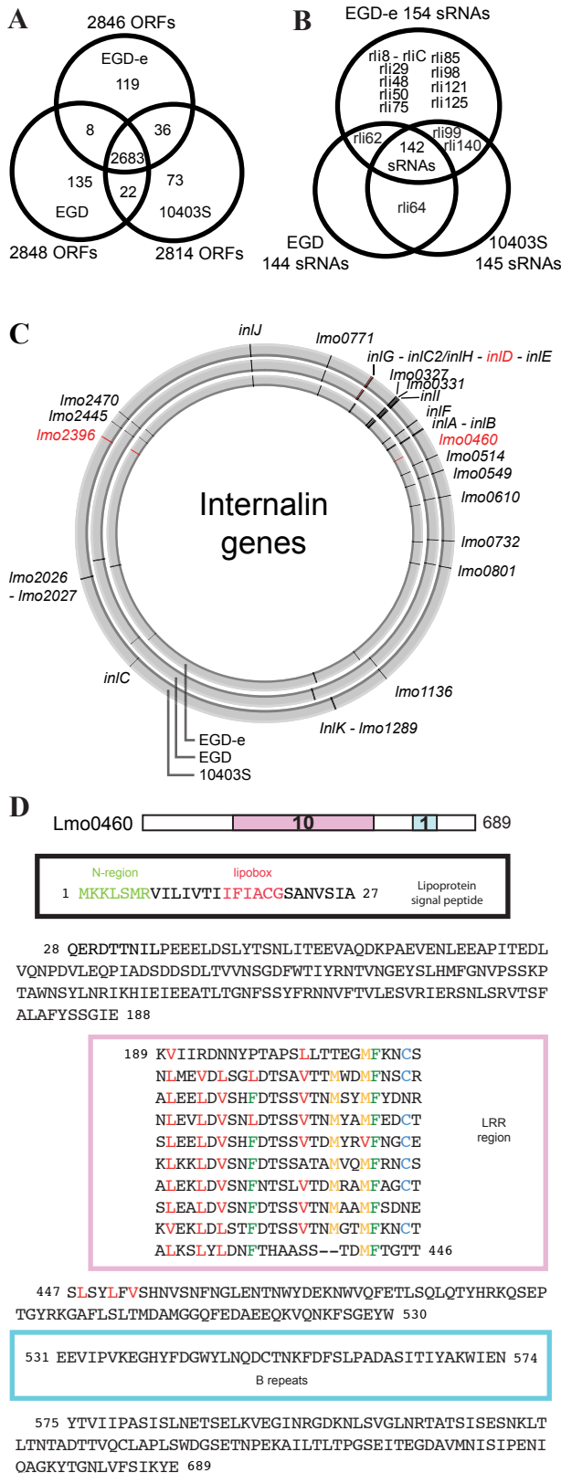
FIG 2 Conservation of ORFs, small RNAs, and internalins in EGD, EGD-e, and 10403S. (A) Venn diagram showing the numbers of ORFs common to the different strains. A bidirectional best-hit search with an E value score lower than 1e-4 was used to determine homologies. (B) Venn diagram of the small RNAs found in the three strains. The percentage of similarity was calculated (Continued)
