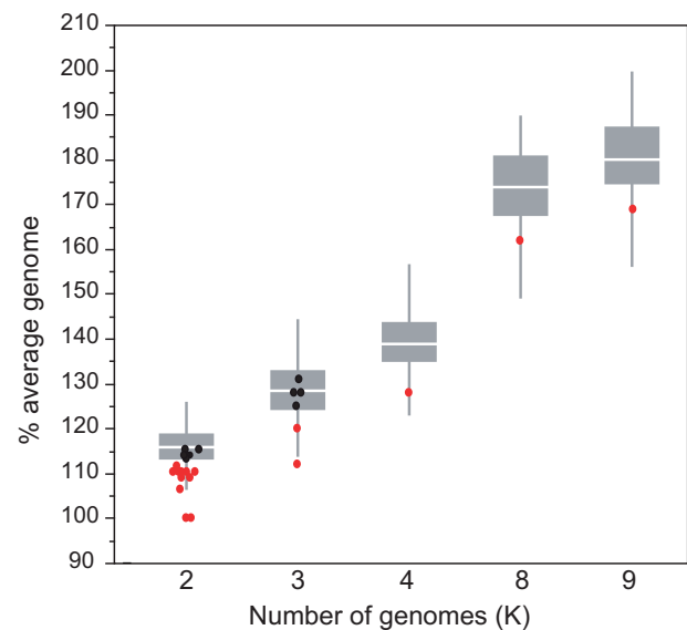
Fig. 2. —Comparisons of the pan-genome of A. baumannii computed with random samples of different size (boxplots) with those of the other species or genomic species. Each species, except A. baumannii , is only represented once, in the graph corresponding to the full number of available genomes for the taxa (e.g., nine genomes for A. lwoffii ). The boxplots show the distribution of the size of the pan-genome of A. baumannii using random samples of K A. baumannii genomes ( K = \{2, 3, 4, 8, 9\} genomes). Black dots correspond to pan-genomes of other species that are within the 25–75 percentiles of the distribution of the pan-genomes of A. baumannii , that is, these are pan-genomes approximately the size of A. baumannii given the same number of genomes. Red dots correspond to species with pan-genomes smaller than 75% of the A. baumannii pan-genomes (see supplementary table S5 , Supplementary Material online, for full data).
