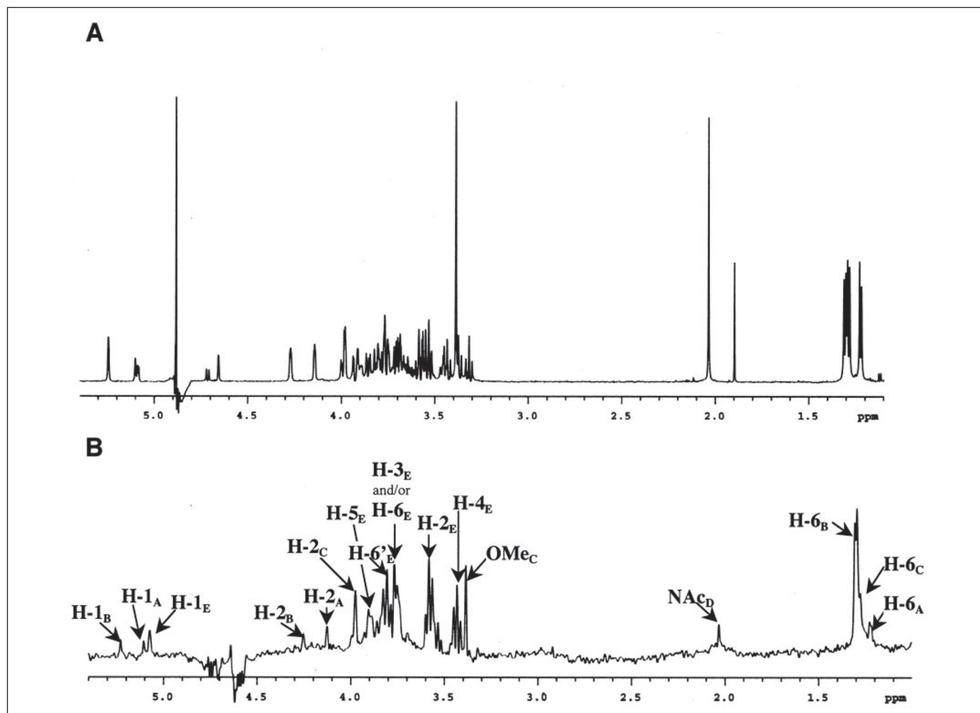
FIGURE 3. mAb binding epitope of the pentasaccharide DA(E)BC-OMe. A , one-dimensional 1 H reference spectrum of pentasaccharide DA(E)BC-OMe in the presence of mlgA C5 (20:1 ratio in site). B , one-dimensional STD-NMR of DA(E)BC-OMe in the presence of mlgA C5 with selective saturation of antibody resonances at 0.3 ppm. Protons of DA(E)BC-OMe affected by the selective saturation of mlgA C5 and so in contact with the mAb are labeled.
