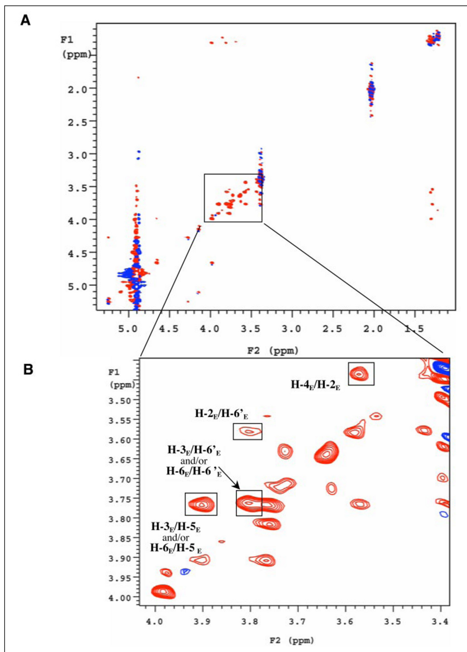
FIGURE 4. The branched glucose residue E of the pentasaccharide DA(E)BC-OMe constitutes a key element in mAb recognition. A , two-dimensional STD-TOCSY of DA(E)BC-OMe in the presence of mIgA C5 (20:1 ratio in site) with selective saturation of antibody resonances at 0.3 ppm. B , a zooming of the two-dimensional STD-TOCSY in the 3.4–4 ppm region emphasizing the glucose E proton connectivities.
