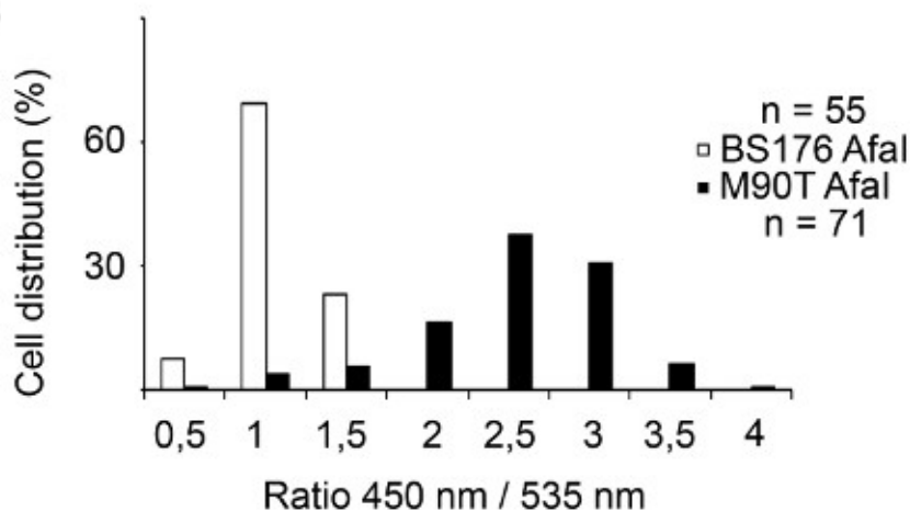
Figure 3. Tracking Shigella flexneri vacuolar rupture in HeLa cells using epifluorescence microscopy. (A) After 2 hr 30 min of CCF4-AM loading, HeLa cells are infected with the \beta -lactamase expressing Shigella flexneri BS176 Afal mutant strain or the M90T Afal virulent strain for 1 hr and fixed using 4% paraformaldehyde for 10 min. Then, cells are imaged using an epifluorescence microscope with a 20x objective. Representative pictures were chosen with the following channels: CCF4 intact probe 535 nm (green) and CCF4 cleaved probe 450 nm (blue). (B) Histogram representing the outcome of our automated analysis on MetaMorph software. The individual cells are distributed in function of their ratio of the intensities in the 450 and 535 nm channels.
