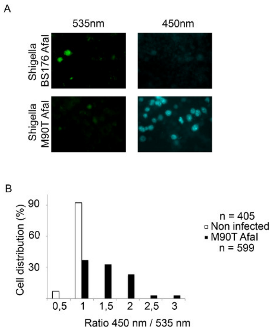
Figure 4. Tracking Shigella flexneri vacuolar rupture in THP-1 cells using epifluorescence microscopy. (A) After 2 hr 30 min of CCF4-AM loading, THP-1 cells are infected with the \beta -lactamase expressing Shigella flexneri BS176 Afal mutant strain or the M90T Afal virulent strain for 1 hr 30 min and fixed using 4% paraformaldehyde for 10 min. Then, cells are imaged using an epifluorescence microscope with a 20x objective. Representative pictures were chosen with the following channels: CCF4 intact probe 535 nm (green) and CCF4 cleaved probe 450 nm (blue). (B) Histogram representing the outcome of our automated analysis using the MetaMorph software. The individual cells are distributed in function of their ratio of the intensities in the 450 and 535 nm channels.
