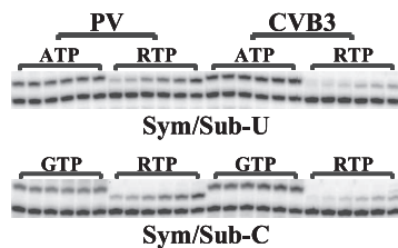
FIG 2 CVB3 encodes an RdRp with higher fidelity than PV. The RdRp from either PV (left) or CVB3 (right) was incubated with sym/sub substrate and either the correct nucleotide substrate or RTP as previously described (3, 15). Panels for each nucleotide correspond to quenching at 30, 60, 120, 300, 600, or 1,800 s.
