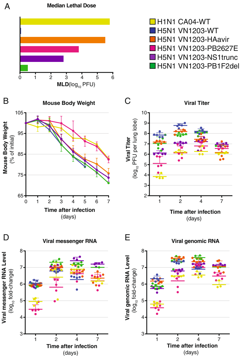
Figure 1 MLD and phenotypical variables collected for all viruses at the 10^4 PFU infection dosage. (A) Median lethal dose (MLD) values of the different viruses in 6-week-old BALB/c mice. MLD values for VN1203 and mutants were performed in one experiment (3 mice per inoculation dosage), and the previously calculated MLD for CA04 is included for comparison [22]. (B) Mice body weight measurements collected each day from 1 to 7 days post-infection for the 10^4 PFU infection dosages. For each virus and time point, the mean and the standard deviation of the mice body weight measurements are indicated by a vertical bar. (C), (D) and (E) Viral titer, viral messenger RNA, and viral genomic RNA measurements collected at 1, 2, 4 and 7 days post-infection for the 10^4 PFU infection dosages. For each virus and time point the set of individual measurements are indicated by filled dots and the mean amongst the individual samples is indicated by a horizontal bar. For the experiments shown in panels B-E, four to five mice were used for all VN1203-WT and pathogenicity mutant infections, while 3–4 mice were used for the CA04 infections. The same animals were used to derive all the phenotypical data (i.e. weight loss, virus titer and virus mRNA/genomic RNA levels).
