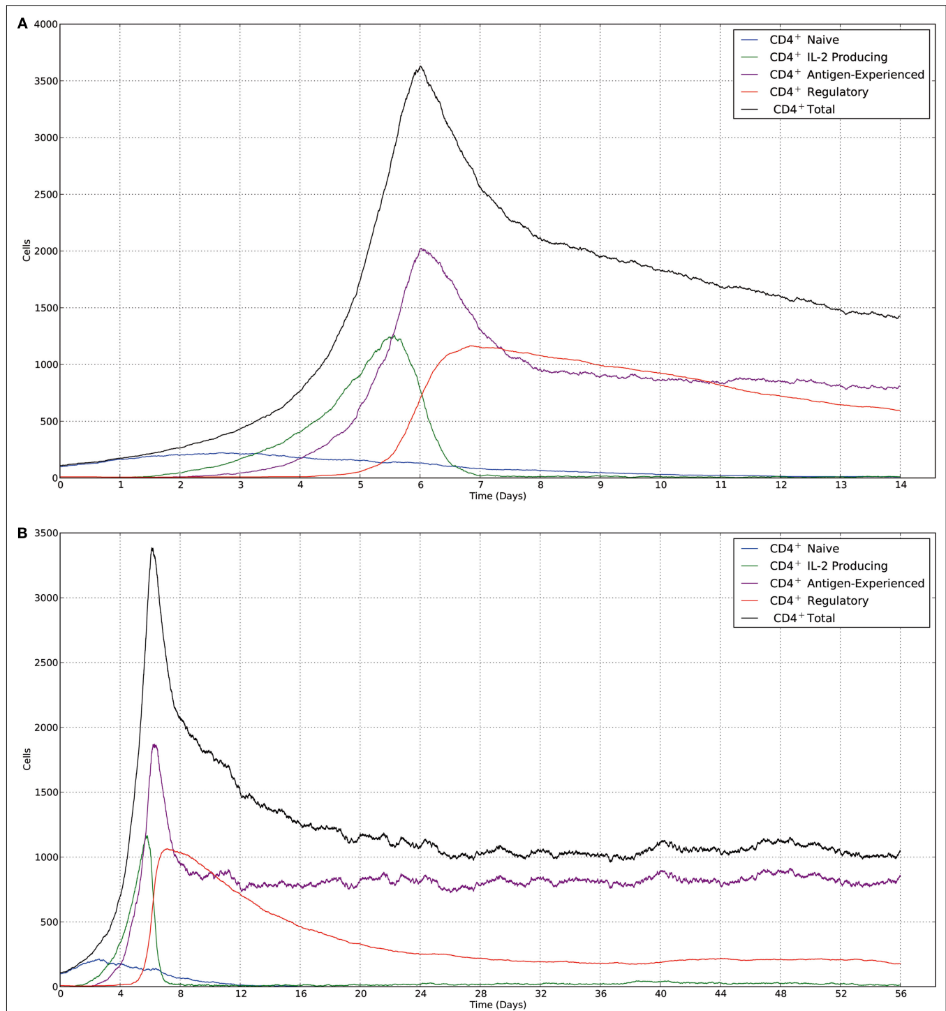
FIGURE 3 | Realizations of the stochastic model carried out using the Gillespie algorithm. All parameters and initial conditions are the same as in the deterministic model, with (A,B), respectively, correlating to (A,B) from
