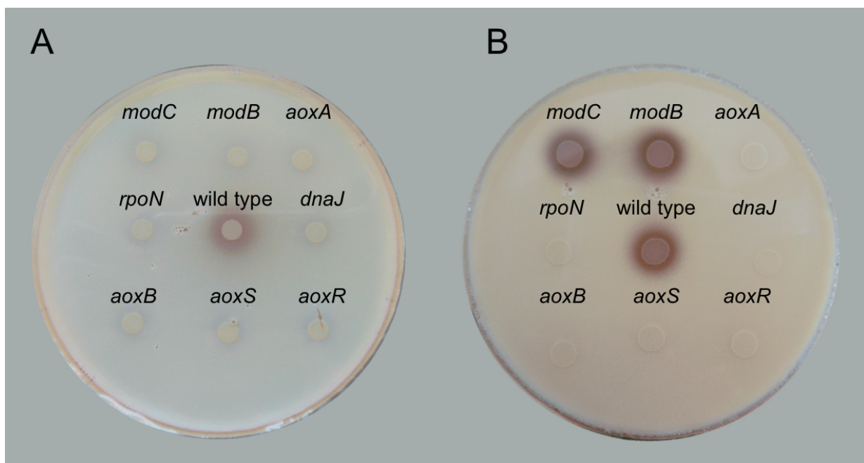
Figure 1 Effect of the various mutations on arsenite oxidase activity. This reaction was tested on plate after silver nitrate staining. Colonies expressing arsenite oxidase activity revealed a brownish precipitate on CDM solid medium. A. Detection of mutants without arsenite oxidase activity after 48 hours incubation on CDM plates. B. Recover of arsenite oxidase activity in modB and modC mutants in the presence of 50 \mu M Mo in the solid CDM medium.
