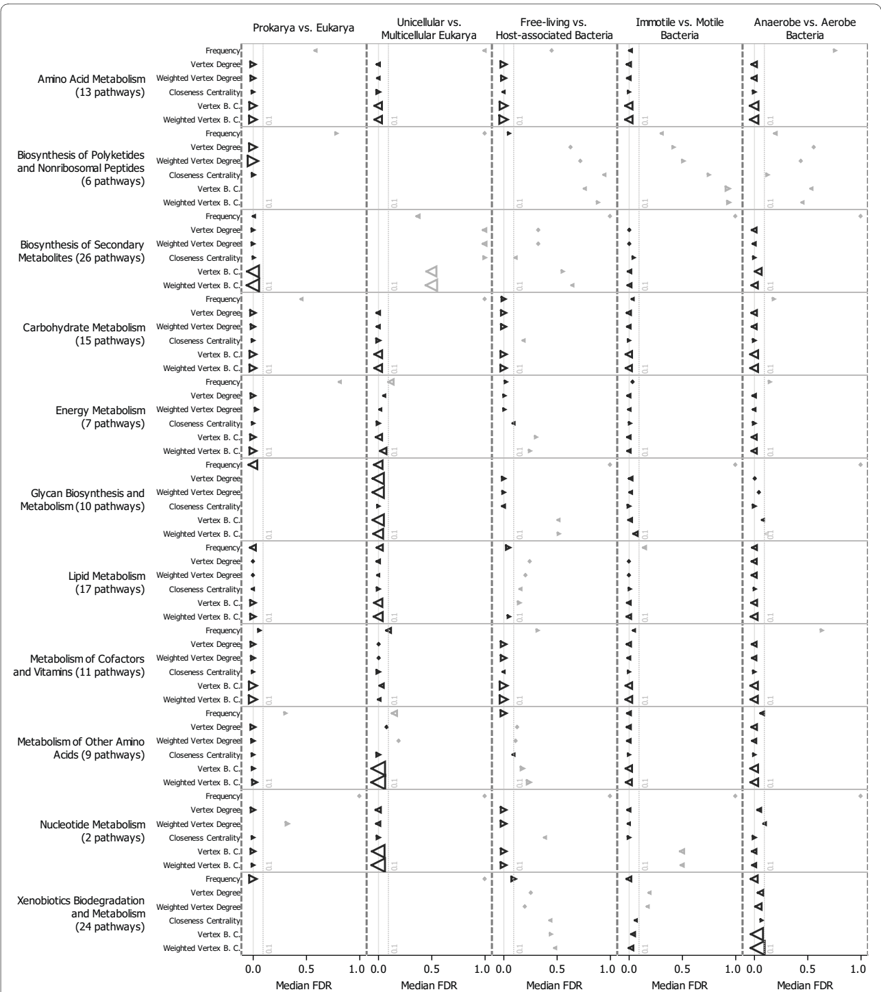
Figure 2 Effects of lineage and environment on pathway frequency, connectivity and centrality. The amplitude of variation of six scores of frequency, connectivity and centrality, and a p-value evaluating the significance of this variation are reported for all metabolic pathways. P-values were calculated by either a Fisher's Exact Test (frequency) or Mann-Whitney U-text (connectivity and centrality), and corrected for multiple testing using the Benjamini-Hochberg method [31]. The median variation and the p-value for pathways in the same functional category were pictured as either a triangle or a diamond. A triangle pointing left (◀) means the score increases from left to right (e.g., from Prokarya to Eukarya), while a triangle pointing right (▶) means the score decreases from left to right. A diamond means the score does not change. The position of the symbol is proportional to the median corrected p-value, i.e. False Discovery Rate, and its size is proportional to the amplitude of variation. All values are available in Additional file 2. B.C.: Betweenness Centrality.
