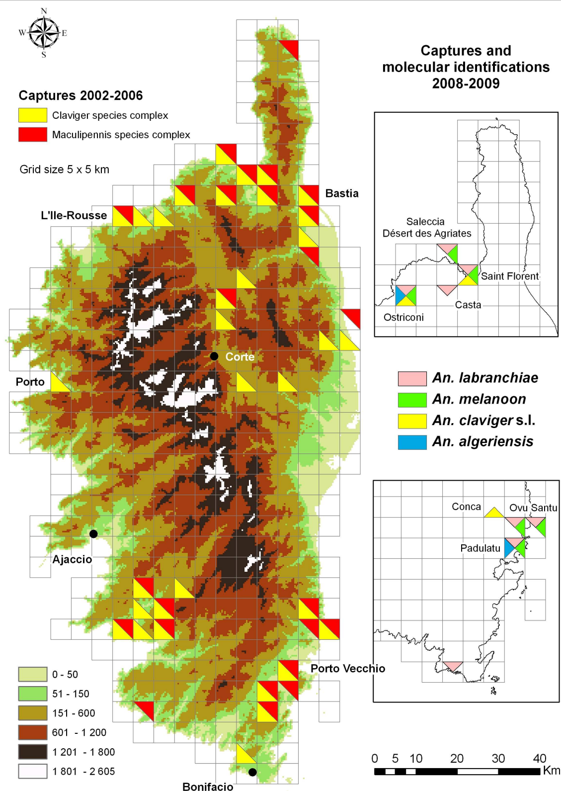
Figure 1 distribution of anophelines belonging to the Claviger and Maculipennis species complexes, based on data captured between 2002 and 2009.
