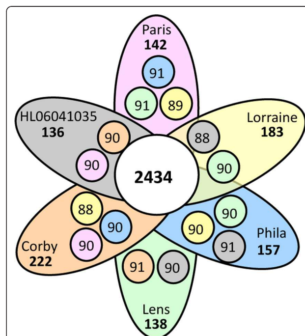
Figure 1 Shared and specific gene content of 6 L. pneumophila genomes. Each petal represents a genome with an associated color. The number in the center of the diagram represents the orthologous genes shared by all the genomes. The number inside of each individual petal corresponds to the specific genes of each genome with non-orthologous genes in any of the other genomes. The small circles inside of each petal represent the percentage of shared genes (total number divided by the number of genes in the smallest genome) between the genome of this petal and the genome represented by the color of the small circle. Yellow circle inside orange petal means that there are 88% of genes shared among Corby and Lorraine.
