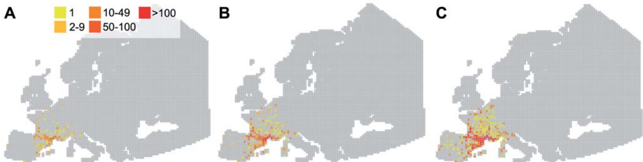
Figure 3. Effect of three virus inactivation rates in water on AIV dispersal during the wintering period (September to January). Hypothetical virus inactivation rates used: A: 7 days; B: 28 days; C: 207 days. Colours represent the number of infectious virus units, on January 31. doi:10.1371/journal.pone.0007289.g003
