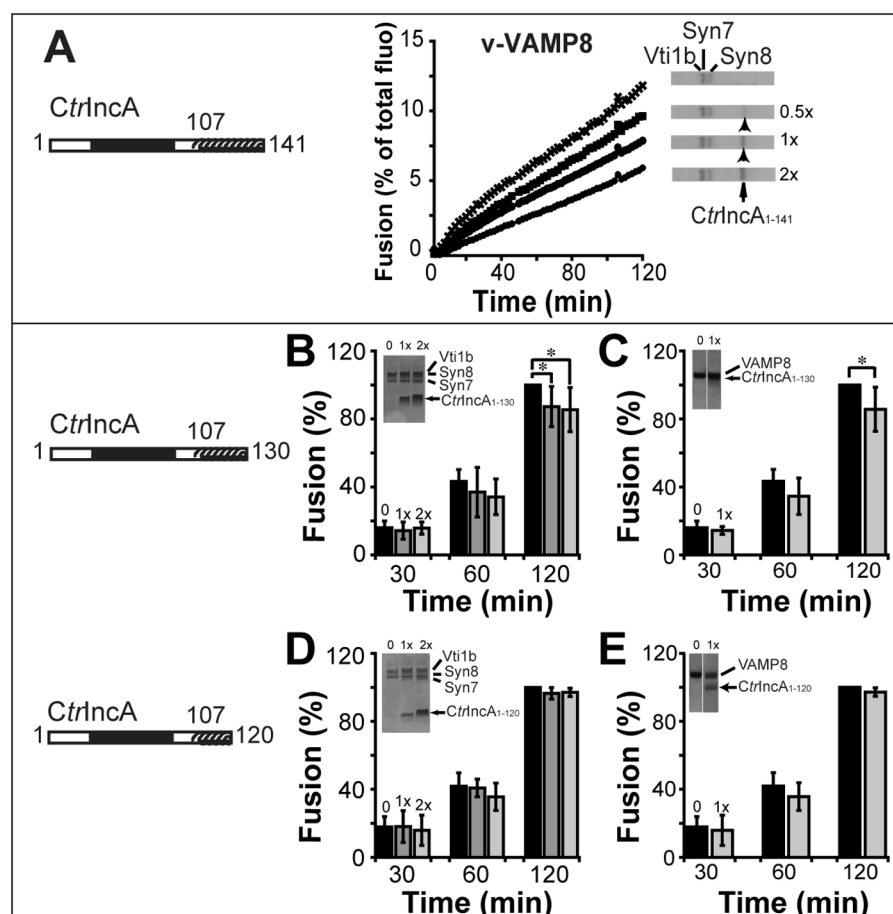
Figure 2. The SNARE-like motif encodes the inhibitory function. A- Increasing concentrations of CtrlIncA 1-141 were reconstituted into endocytic t-SNARE liposomes, and fusion proceeded in presence of VAMP8-liposomes. Fusion is significantly inhibited by the presence of CtrlIncA 1-141 and is dependent upon its concentration, reaching 55% of inhibition after 2 hrs with an estimated CtrlIncA 1-141 :SNARE ratio of 2:1. This experiment is representative of n =3. B-E- Two different concentrations of truncated CtrlIncA (see representative coomassie gels inserted in each graph) were reconstituted into t-SNARE (B,D), and v-SNARE liposomes (C,E). As shown on graphs B and C, CtrlIncA 1-130 still displays a significant inhibitory effect on the endocytic SNARE-mediated membrane fusion (average of 15% inhibition after 2 hrs, p =0.022). On the contrary, CtrlIncA 1-120 (D,E) completely fails to inhibit endocytic fusion ( p >0.05). The mean from n =5 independent experiments was determined at 30 min, 60 min and 120 min. The standard deviation is shown. One asterisk denotes statistically significant differences ( p <0.05). For the purpose of comparison, maximal values of fusion obtained for the SNARE complex without IncA at 120 min were arbitrarily defined as 100%. doi:10.1371/journal.pone.0007375.g002
