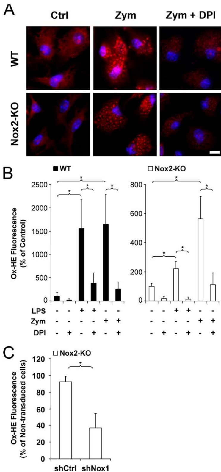
Figure 4. Contributions of Nox1 and Nox2 to intracellular O_2^{\cdot-} levels in activated microglia. A , B , Cultured WT and Nox2-KO microglia were incubated for 45 min with cell-permeant hydroethidine in the absence (Ctrl) or the presence of LPS or zymosan and with or without DPI before assessment of hydroethidine oxidation. A , Red fluorescence resulting of hydroethidine oxidation in cells that have ingested zymosan. Strongly enhanced fluorescence is localized in phagosomes containing zymosan in WT or Nox2-KO cells. Fluorescence is strongly reduced when cells are incubated with DPI. Hoechst 33342 dye counterstaining (blue) reveals cell nuclei. Scale bar, 10 \mu m. B , Levels of oxidized hydroethidine (Ox-HE) were determined by fluorescence intensity normalized to the number of cells and are expressed as the percentage of the mean control value determined in cultures without LPS, zymosan or DPI. In zymosan-treated cultures, Ox-HE levels were determined in cells containing at least 10 zymosan particles. Data are the mean \pm SD of two (Nox2-KO cells) or three (WT cells) separate experiments with 5–15 determinations in sister wells
