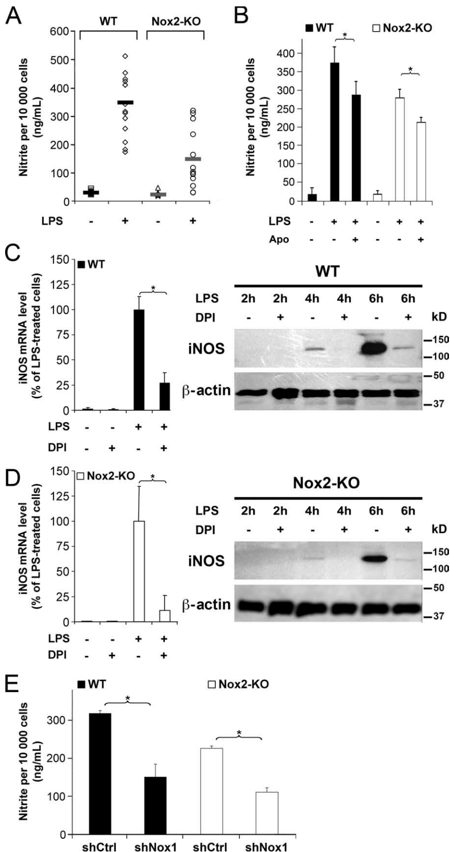
Figure 6. Both Nox1 and Nox2 promote microglial production of NO. A, B , Cell production of NO \cdot was determined by colorimetric measurement of nitrite levels in the medium of WT or Nox2-KO microglial cultures treated or not with LPS or LPS and apocynin for 16 h. A , Dots represent mean values in 15 WT and 13 Nox2-KO independent experiments (5–6 determinations in sister wells per experiment). Bold lines indicate the mean value calculated from the means of the independent experiments. B , For each genotype, data are mean \pm SD of six determinations in sister wells from a representative experiment (* p < 0.01, SNK test). C, D , Real-time PCR determination of iNOS mRNA levels and Western blot detection of iNOS protein in WT ( C ) or Nox2-KO ( D )
