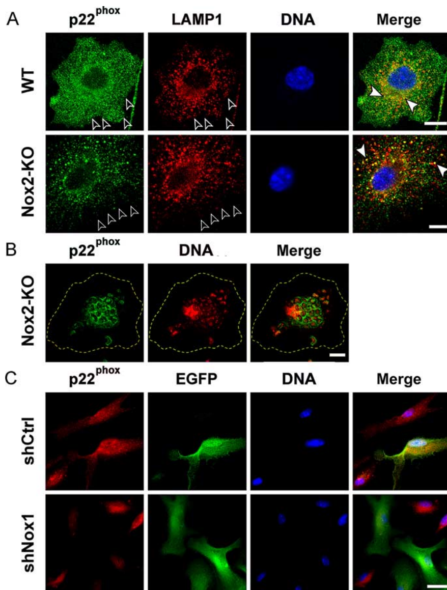
Figure 2. Nox1- and Nox2-dependent localization of p22 phox in microglia. A , Codetection of p22 phox (anti- p22 phox , green), lysosomes (anti-LAMP1, red), and nuclei (Hoechst 33342, blue) in cultured WT or Nox2-KO microglia. Plasma membranes are outlined by open arrowheads. White arrowheads point to lysosomal p22 phox in merged views (confocal microscopy). Scale bars, 10 \mu m. B , Detection of p22 phox (green) and nucleic acid (Hoechst staining, blue fluorescence converted to red) in a Nox2-KO murine microglial cell after microglial phagocytosis of yeast particles (zymosan). The plasma membrane is outlined in yellow. Cultured cells were incubated with zymosan for 45 min before fixation and staining. Note the localization of p22 phox in phagosome membranes surrounding stained nucleic acid of yeast particles (confocal microscopy). Scale bar, 10 \mu m. C , Suppression of p22 phox expression in Nox2-KO microglial cells transduced with shNox1. Cultures of purified Nox2-KO microglia were transduced with lentiviral shNox1 or shCtrl and cultured for 3 d before fixation and codetection of p22 phox (anti- p22 phox , red) and EGFP (anti-EGFP, green). Cells transduced with lentiviral shRNA express EGFP. Scale bar, 20 \mu m.
