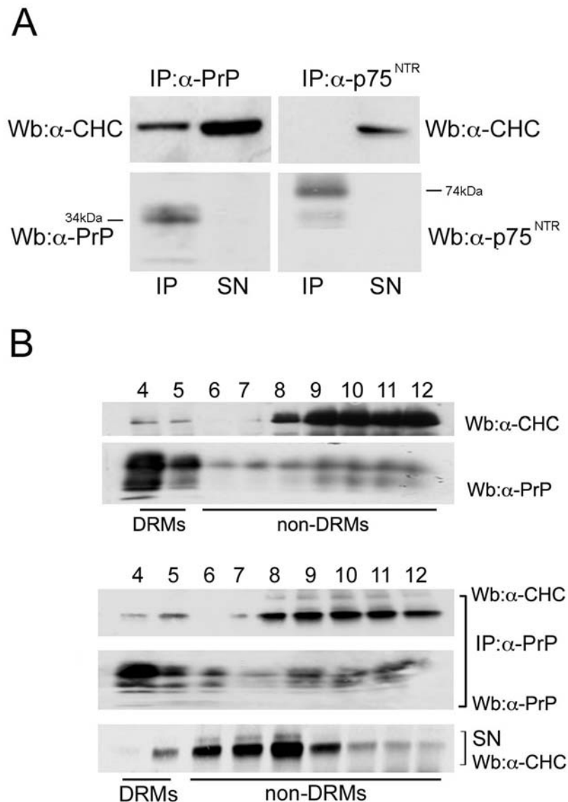
Figure 6. PrP C and clathrin co-immunoprecipitate both in DRM and non-DRM fractions. A) FRT-PrP C cells grown on filters were lysed, immunoprecipitated (IP) by \alpha PrP antibody (SAF32) or \alpha p75 NTR antibody (as negative control), and revealed using: \alpha CHC (TD.1) or \alpha PrP and \alpha p75 NTR antibody as indicated. The supernatants (SN) of the immunoprecipitates were tested by western blot to verify the efficiency of the coimmunoprecipitation. B) Filter grown FRT-PrP C cells were lysed and run on OptiPrep TM gradient to separate DRM from non-DRM fractions. The relative distribution of CHC and PrP C in the fractions (upper panel) was tested by western blot of an aliquot of gradient fractions with specific antibodies. The remaining amount of each fraction (bottom panel) was immunoprecipitated with \alpha PrP antibody SAF32 and revealed by \alpha CHC TD.1 antibody. Supernatants (SN) of the immunoprecipitation (IP) are shown in the bottom panel. doi:10.1371/journal.pone.0005829.g006
