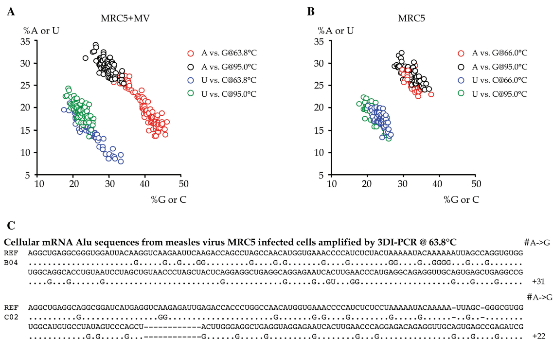
Figure 5. Selective amplification of ADAR-edited Alu elements nested in cellular mRNAs. (A) A versus G base composition (red and black) and U versus C (blue and green) of individual Alu sequences from cellular mRNAs from measles virus (MV) infected MRC-5 cells. Sequences were derived at standard (95°C, n=77 sequences) and restrictive temperatures (63.8°C, n=108 sequences). A versus G correlations pertain to plus sense Alu sequences (%A = -0.996\%G + 59.8 ; r=0.915 , n=108 , P<10^{-3} ) and U versus C (%U = -0.922\%C + 38.1 ; r=0.914 , n=108 , P<10^{-3} ), the anti-sense. The two gradients indicate a strict interconversion of A to G and U to C. (B) A versus G and U versus C correlations for Alu sequences derived from cellular mRNA from uninfected MRC5 cells under normal ( n=58 sequences) and 3DI-PCR ( n=67 sequences). (C) Two examples of highly edited Alu elements (B04 and C02) nested within cellular mRNAs. The alignments were those of the best hits derived from blasting the human genome. Only differences are shown to emphasize the effects of ADAR editing. Gaps were introduced into the C02 sequence to allow comparison with the B04 alignment. The number of A→G transitions are shown to the right.
