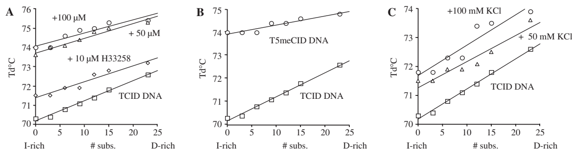
Figure 2. The temperature differential of TCID DNA is relatively refractory to manipulation. (A) Hoechst bisbenzimidazole dye H33258 that binds to AT-rich DNA via the minor groove increases the Td but not the temperature differential. (B) Substituting modified bases such as 5-MedCTP for dCTP, dUTP for dTTP and 7-deazadGTP for dGTP (not shown) also failed to increase the temperature differential of TCID DNA. (C) Increasing the ionic strength by the addition of monovalent (K + ) and divalent cations (Mn 2+ , not shown) failed to increase the temperature differential.
