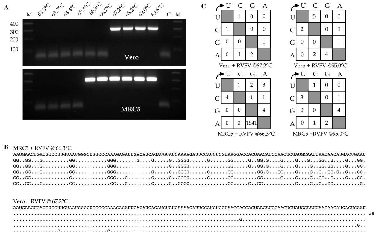
Figure 4. Massive adenosine deamination of Rift valley fever virus genomes. RVFV clone 13 is a highly immunogenic yet attenuated strain that encodes a 549 bp in frame deletion within the NSs gene. As the vestigial NSs protein has lost its ability to antagonize interferon production, clone 13 is a good inducer of interferon, unlike virulent strains (47). While clone 13 grows well on Vero cells, viral titres were 100-fold lower on MRC-5 cells. (A) Agarose gel of TCID DNA amplified from RVFV infected Vero and MRC-5 cells. The PCR products amplified from the latter between 66.3 and 66.7°C are indicative of genomes enriched in GC. C, negative buffer control; M molecular weight markers. (B) RVFV sequences derived from amplification at the lowest denaturation temperature (66.3°C). Sequences are aligned to the reference MV sequence, only differences being shown. The monotonous A→G transitions are typical of ADAR editing. Complete sequence sets are given in Supplementary Figure 4. (C) Mutation matrices for the sequence sets. The number of sequences per matrix is, starting top left and going clockwise n = 6, 10, 11 and 26. The symmetry of the matrices 95°C amplification controls is typical of a viral quasispecies.
