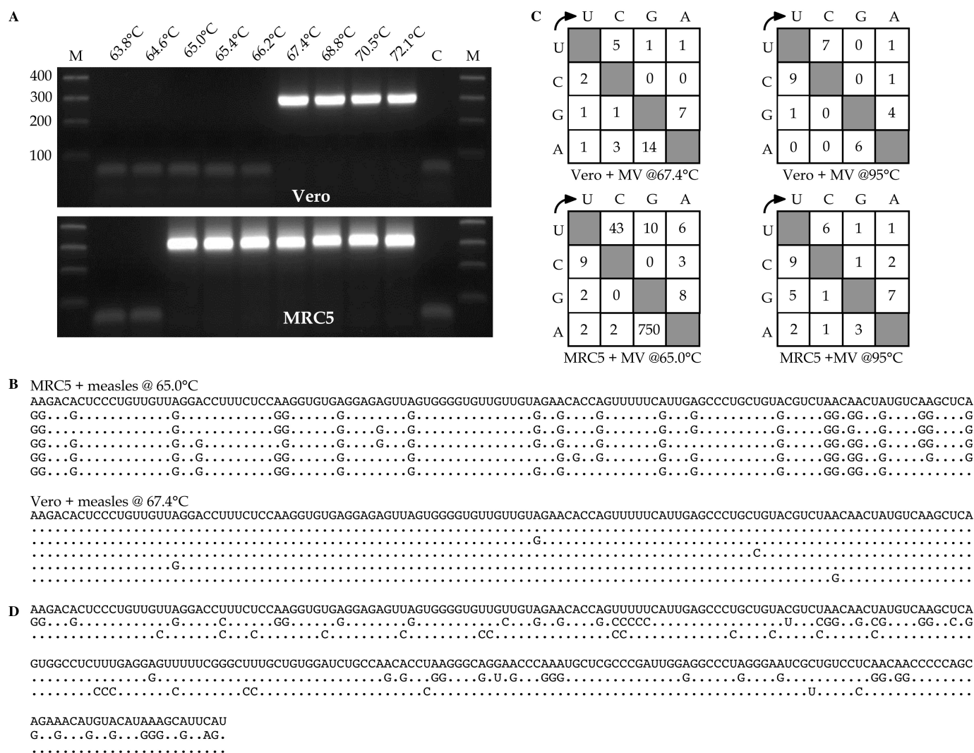
Figure 3. 3DI-PCR amplification of ADAR edited measles virus genomes. (A) Agarose gel of TCID DNA amplified from measles infected Vero and MRC-5 cells. The PCR products amplified from the latter between 65 and 66.2°C are indicative of genomes enriched in GC. C, negative buffer control; M molecular weight markers. (B) MV sequences derived from amplification at the lowest denaturation temperature (65°C). Sequences are aligned to the reference MV sequence, only differences being shown. The monotonous A→G transitions are typical of ADAR editing. Complete sequence sets are given in Supplemental Figure 2. (C) Mutation matrices for the sequence sets. The number of sequences per matrix is, starting top left and going clockwise n = 15, 13, 21 and 19. The symmetry of the matrices 95°C amplification controls is typical of a viral quasispecies. A slight skew in the Vero/MV 67.4°C matrix from AU→GC is understandable given that 3DI-PCR amplifies GC-rich sequences, and represents the GC-rich end of the mutant spectrum. (D) Sequences of two C-rich MV sequences compared to the reference genome. The first encodes A→G and U→C transitions and arises from editing of the viral genome and anti-genome, while the latter U→C transitions indicating editing only of the anti-genome.
