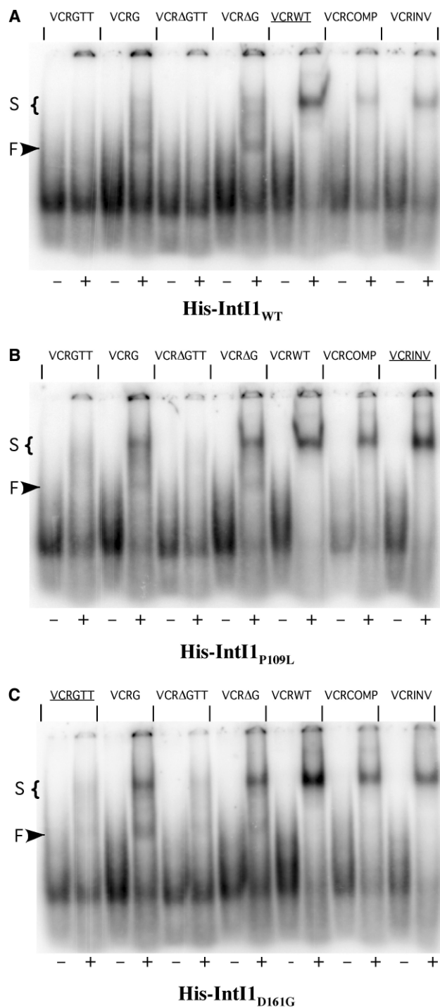
Figure 4. Gel retardation of bs VCRd derivatives by (A) His- IntI1 WT (B) His- IntI1 P109L and (C) His- IntI1 D161G . The substrate that the respective mutant was selected on is underlined. 0.6 pmol of each probe and 1500 nM of protein were used in each reaction. In the lanes marked with -, no protein was added. Faster (F) and slower (S) complexes are indicated by arrows.
