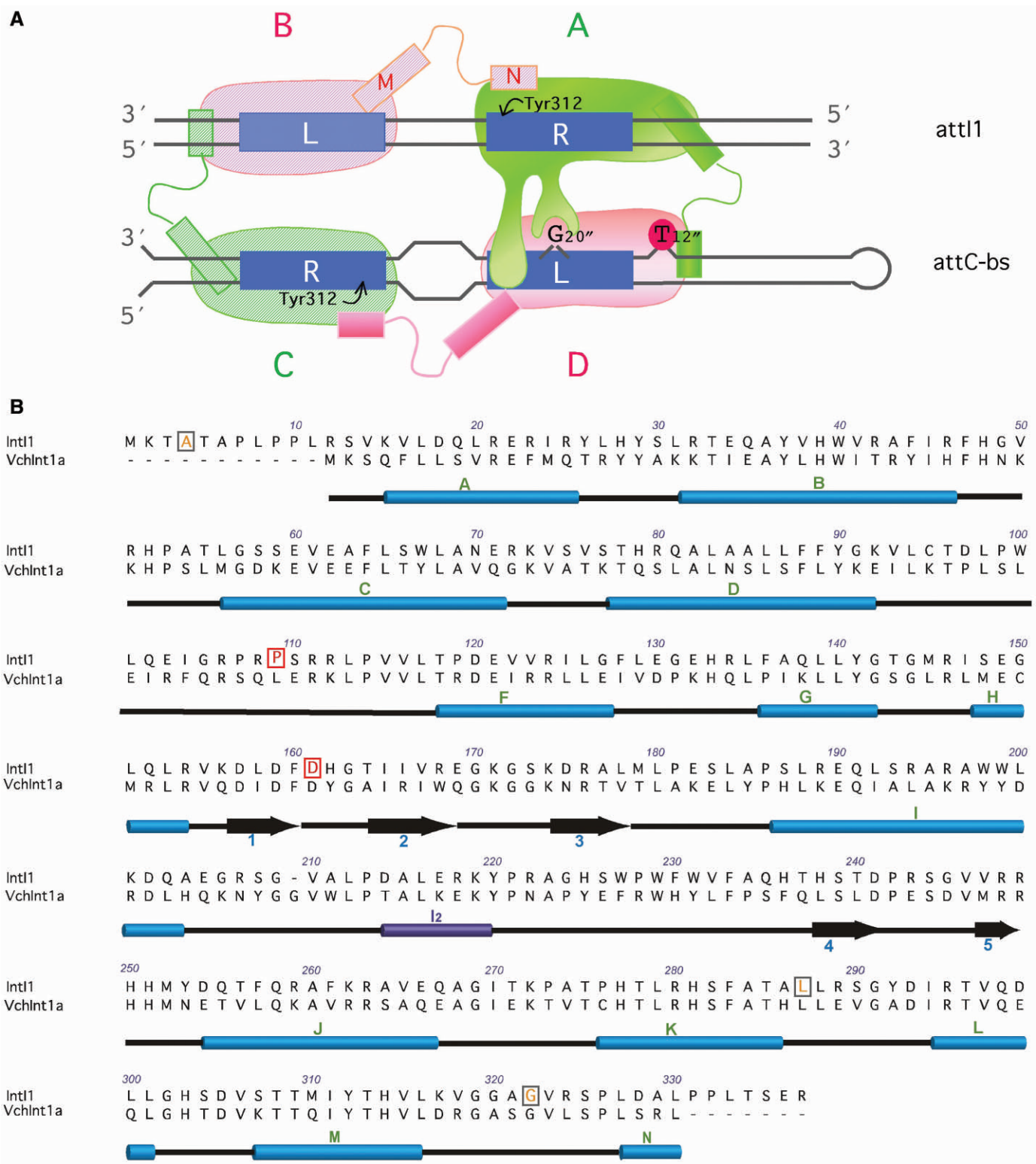
Figure 6. (A) A schematic picture of the IntI1 synapse with attC × attI1 . Subunits B and C are striped since the positioning of these molecules cannot be predicted from the crystal structure of the VchIntIA, made from an attC × attC recombination complex. (B) Alignment of the protein sequences from IntI1 and VchIntA. The residues carried by the mutants selected by the enrichment assay are in frame. Those selected on the mutated attC VCR substrates are in bold, red and with a red frame. The secondary structure of VchIntIA with the β-strands (arrows) and the α-helices (cylinders) is presented below the sequence alignment.
