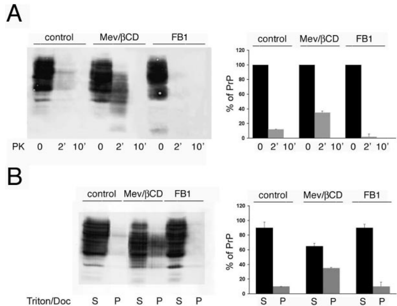
Figure 6. Analysis of PrP C misfolding in FRT cells. FRT cells were grown in 35-mm dishes in control (control), cholesterol (Mev/ \beta CD), or sphingolipid (FB1) depletion conditions. The cells were lysed in Triton/Doc buffer, in the absence of proteases inhibitors, and where indicated were treated with PK (3.3 \mu g/ml) for 2 or 10 min (A) or centrifuged in a TLA 100.3 rotor at 265,000 \times g and separated into soluble (S) and insoluble (P) materials (B). In both cases PrP C was revealed by Western blotting by using specific antibodies and ECL. The data were also quantified using the NIH image program for Macintosh and plotted as indicated in the graphs on the right panels. Error bars are indicated.
