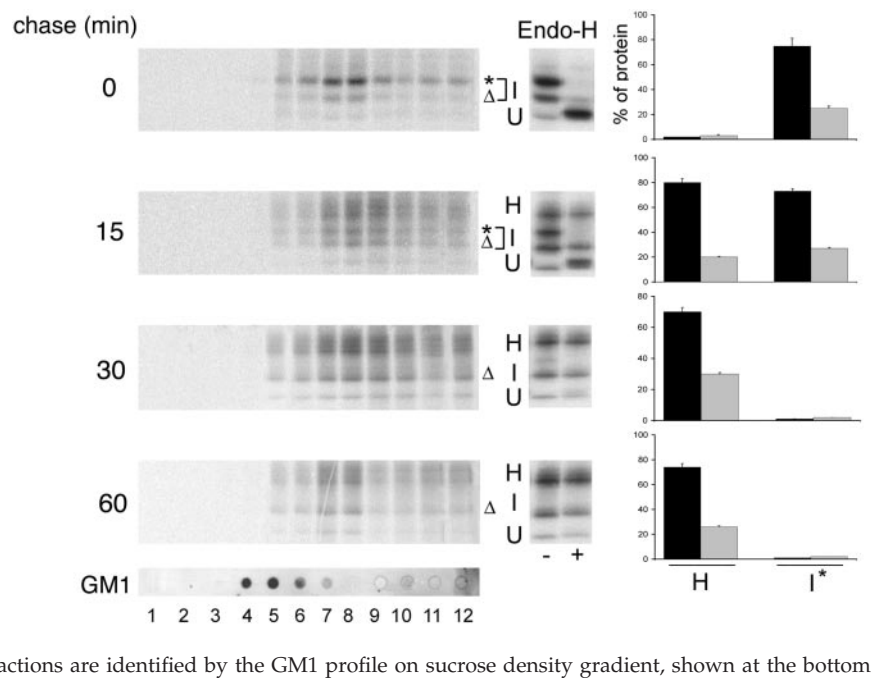
Figure 2. Association of PrP C with DRMs in the early secretory pathway. FRT cells grown on 100-mm dishes (3 dishes for each chase time) were pulsed for 20 min with [ 35 S]methionine and then chased for the indicated times. The cells were lysed in TNE/TX-100 1% buffer and then run through a linear 5–40% sucrose gradient. One-milliliter fractions were collected from the top to bottom of the tube after centrifugation to equilibrium, and PrP C was immunoprecipitated from all fractions with SAF 32 antibody and subjected to SDS-PAGE and phosphorimager scanning (left panel). The amount of PrP C in each fraction was quantified by scanning three independent gels using the NIH image software for Macintosh and is represented in right panel as percentage of the total amount of the protein (gray bars indicate the amount of floating PrP C , fractions 1–7; black bars indicate the amount of soluble PrP C , fractions 8–12). Endo-H treatment (Thotakura and Bahl, 1987), performed after every chase time on an aliquot of the sample before running the sucrose gradient, is shown in the middle panel. Error bars are indicated. H, mature, highly glycosylated PrP C isoform; I*, unmodified diglycosylated isoform; I Δ , monoglycosylated form; U, unglycosylated form. Raft fractions are identified by the GM1 profile on sucrose density gradient, shown at the bottom of the picture.
