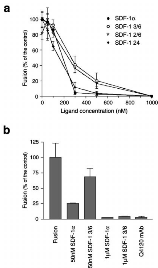
FIG. 2. Comparative analysis of the capacity of SDF-1 \alpha and SDF-1 3/6 and 2/6 mutants to prevent the fusogenic activity of X4 HIV Env. a , cell-to-cell fusion experiments were performed by co-culturing HeLa CD4+ cells carrying an integrated HIV-LTR-driven \beta -gal reporter gene, with HeLa 243 cells co-expressing both the tat and env genes from the pLai X4 HIV-1 proviral molecular clone. After fusion, Tat protein induces in trans the transcription of an HIV-LTR-driven \beta -gal reporter gene. The enzymatic activity detected in the cell lysates reflects the magnitude of the Env-mediated cell fusion. b , cell-to-cell fusion experiments using CXCR4+ activated human PBMC against BHK-21 cells expressing the Env of the X4 HIV-1 Lai isolate. PBMC and BHK-21 cells were loaded with CMTMR and aqueous calcein-AM chromophores, respectively, and cell fusion was quantified by detection of cells simultaneously carrying both markers. All data are mean \pm S.E. of triplicates. Results from one experiment out of three are shown.
