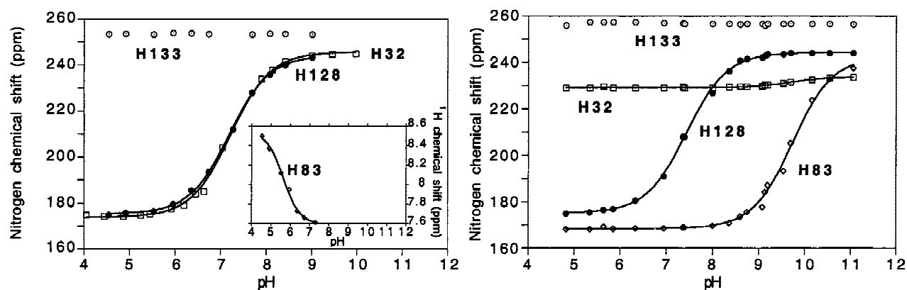
Fig. 2. Heme pocket histidine 15 N chemical shifts of HasA SM for the apo-form (left) and for the holo-form (right) as a function of pH. The solid lines represent the least-squares best fit to the data. The titration curve for the His 83 1 H resonance in the apo-HasA SM is shown in the bottom right corner because only partial 15 N titration curves didn't allow to determine the pK a value by fitting the data for this residue.
