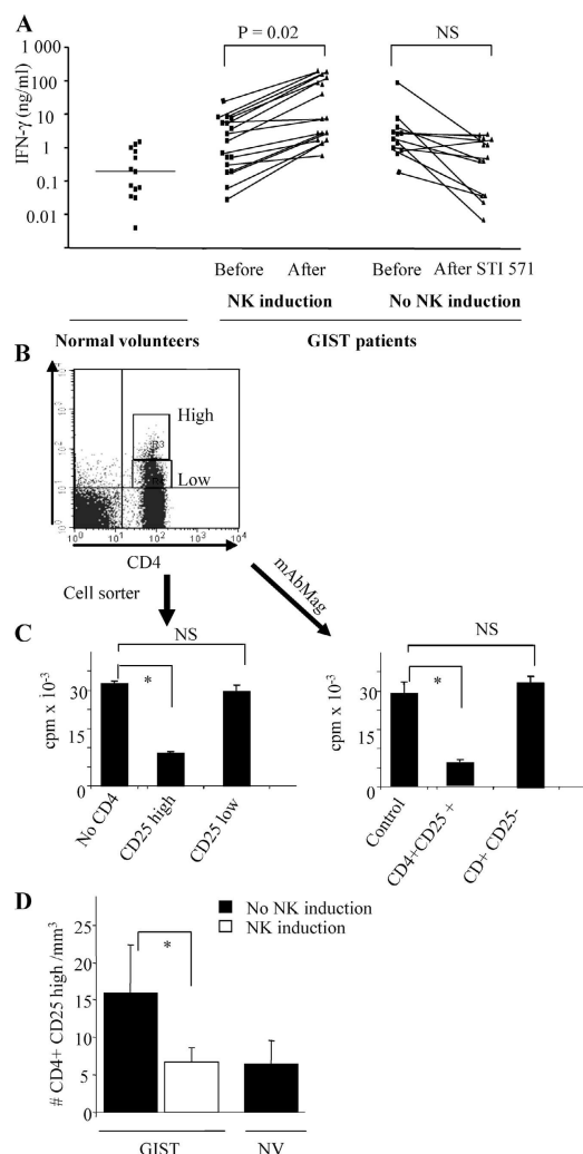
Figure 1. Inverse correlation between T reg cell numbers and NK cell induction in GIST patients treated with imatinib mesylate.
